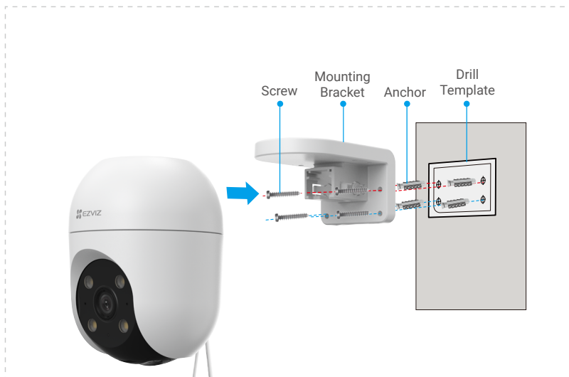
Fig. 2 Wall Mount
